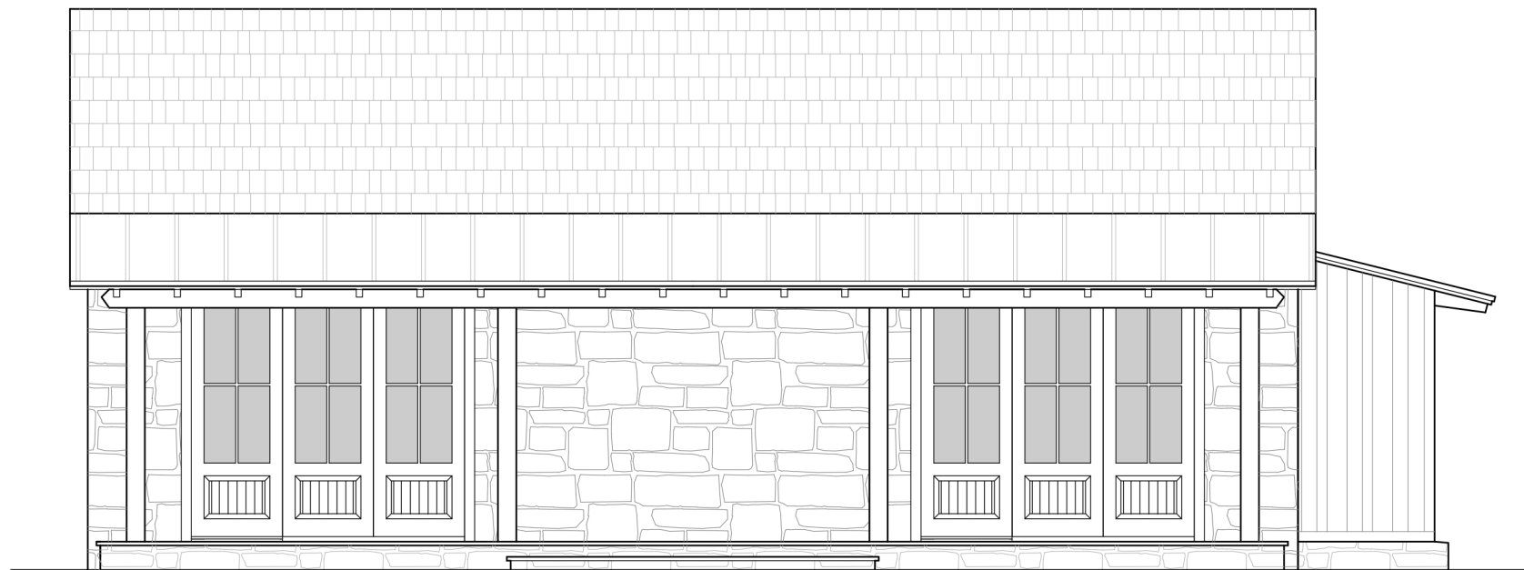
GUEST CABIN - FRONT ELEVATION
