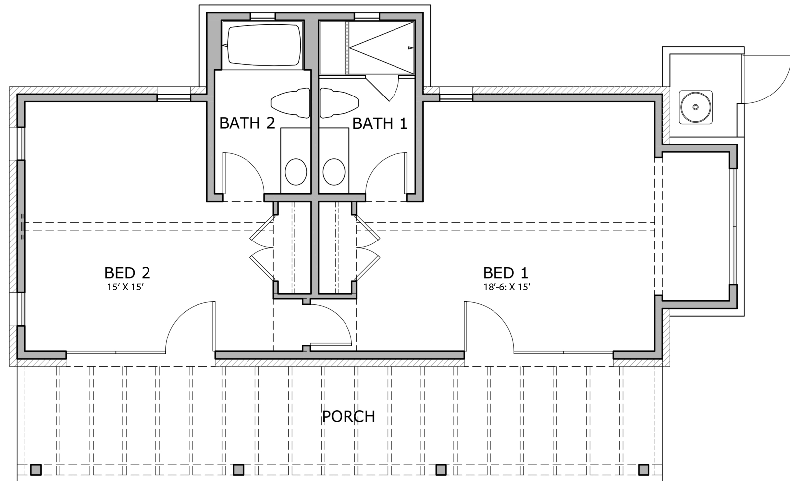
GUEST CABIN - FLOOR PLAN
